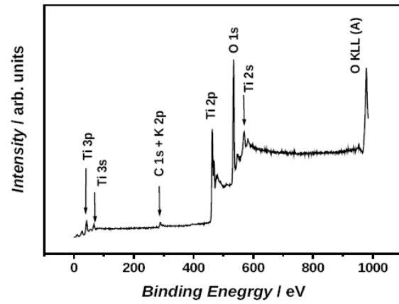
Figure 4: Survey (1000 eV) XP spectrum of TiO 2 fibers
