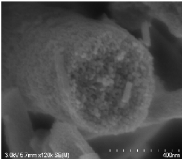
Figure 2: SEM picture of fiber cross section demonstrating polycrystalline fibre character
