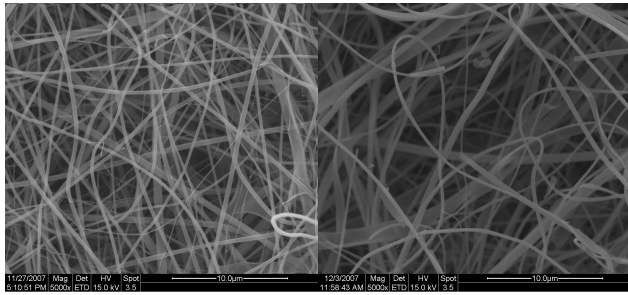
Figure 1: SEM picture of electrospun titania precursor (left) and calcined TiO 2 nanofibers (right)
